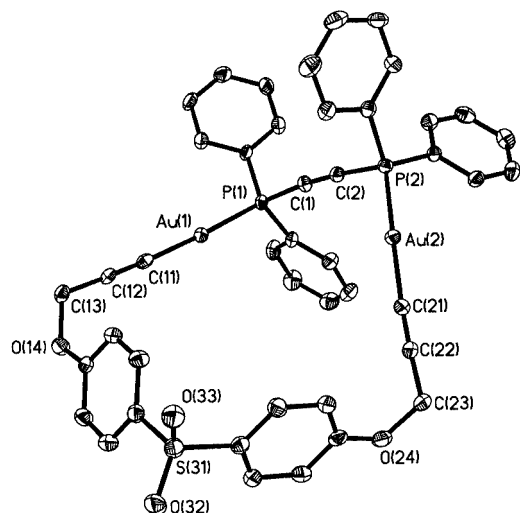
Figure 3. Molecular structure of complex 3a ; ellipsoids show 50% probability levels, hydrogen atoms have been omitted for clarity
