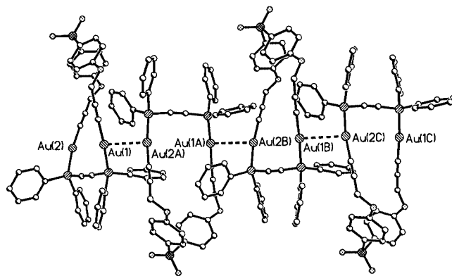
Figure 6. Packing of complex 3a to form a polymeric chain
