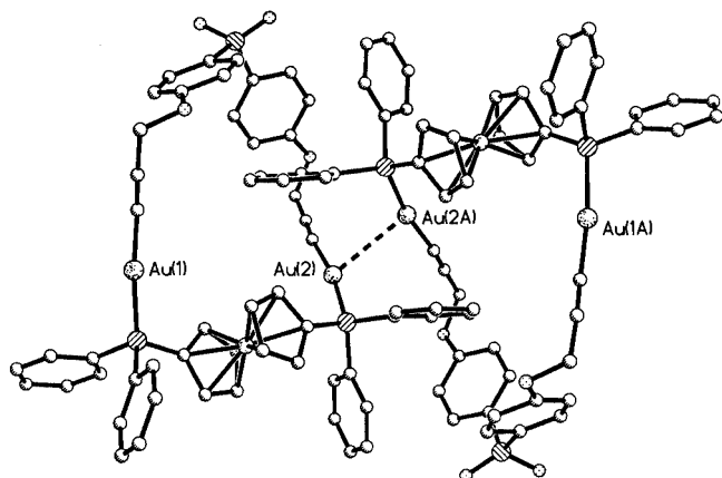
Figure 7. Packing of complex 3d to form dimeric units
