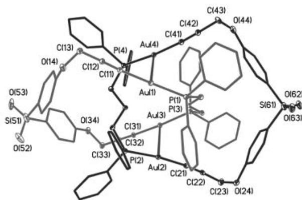
Figure 8. Molecular structure of complex 4a ; ellipsoids show 25% probability levels, \text{C}_6\text{H}_4 and phenyl rings are shown as lines and hydrogen atoms have been omitted for clarity
