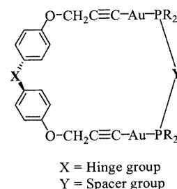
Figure 1. Schematic diagram of a macrocyclic gold(I) complex
