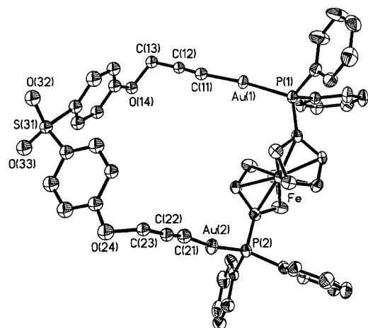
Figure 4. Molecular structure of complex 3b ; ellipsoids show 50% probability levels, hydrogen atoms have been omitted for clarity
