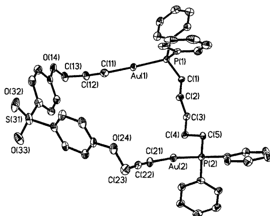
Figure 5. Molecular structure of complex 3d ; ellipsoids show 50% probability levels, hydrogen atoms have been omitted for clarity.
