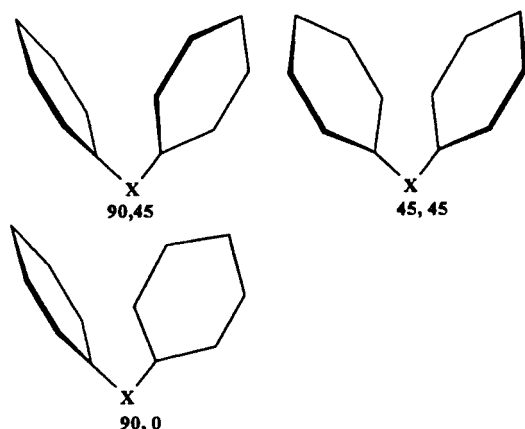
Figure 2. Orientation of aryl groups at the hinge atom X
